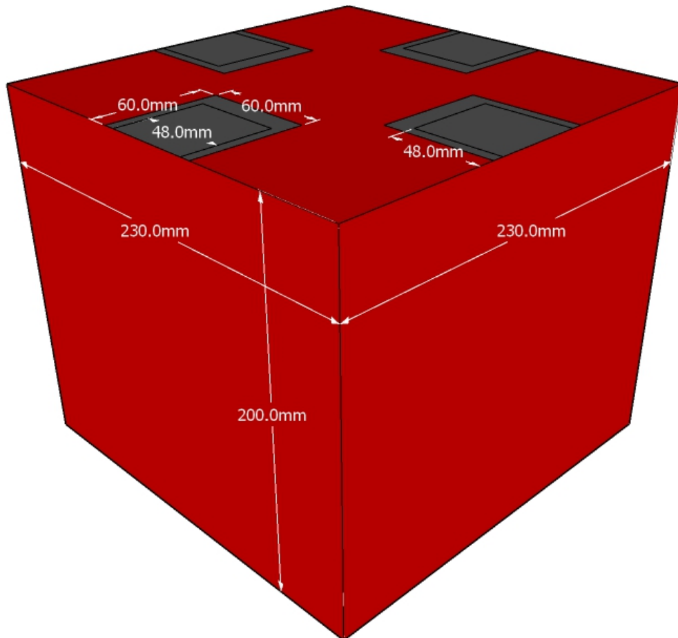
Figure 12. Box's dimensions.
