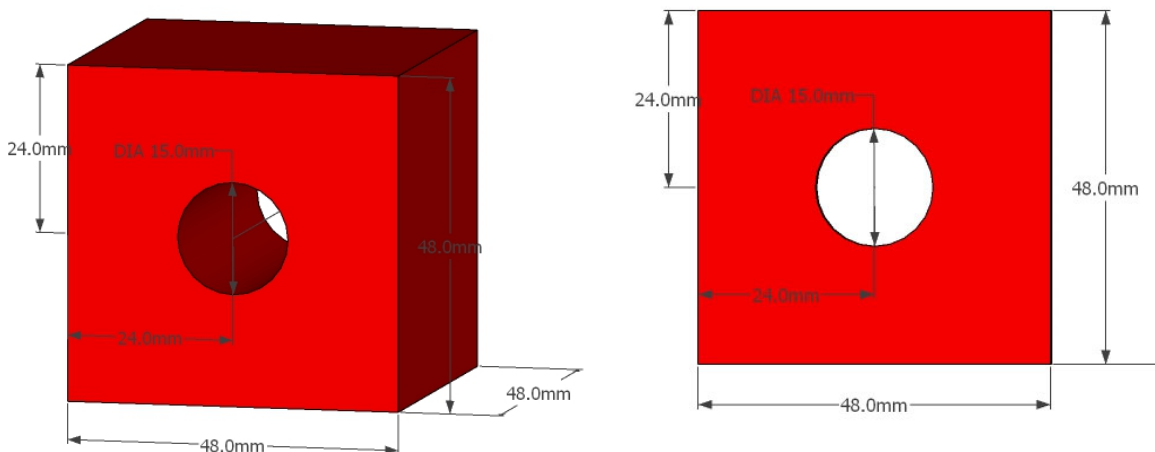
Figure 13. Cube's dimensions.
