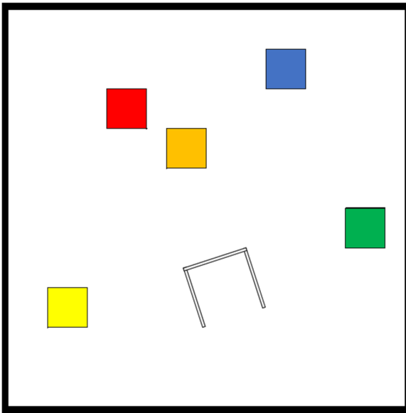
Figure 22. Locations of elements: (K,Q,J,N)(I,I,K,G)(N,C,P,E)(E,O,C,Q).
