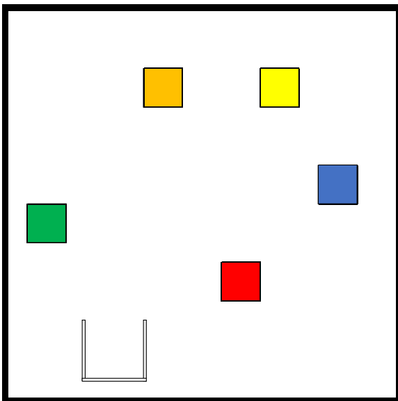
Figure 25. Locations of elements: (H,Q,H,T)(P,D,N,F)(L,N,N,P)(S,K,Q,I).
