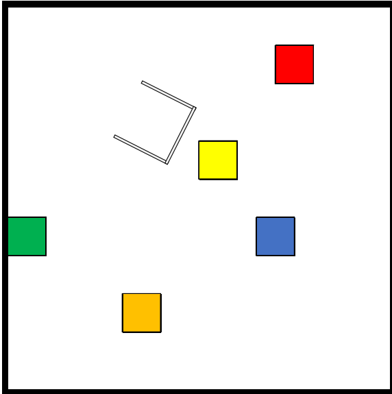
Figure 24. Locations of elements: (H,E,J,F)(N,L,P,N)(O,E,Q,C)(A,L,C,N).
