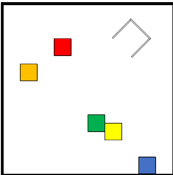
Figure 23. Locations of elements: (N,E,P,C)(M,P,K,N)(C,J,E,H)(Q,S,S,U).
